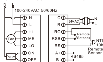
Application 6: 2 pipe/3 wire fan coil system
