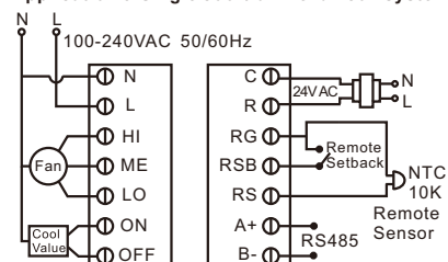
Application 8: Single cool / 3 wire fan coil system
